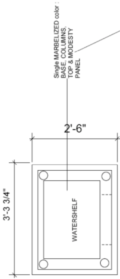
PLAN : LECTERN 1/2" = 1'-0"
